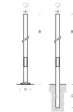
Wood system building element pole · Direct burial
