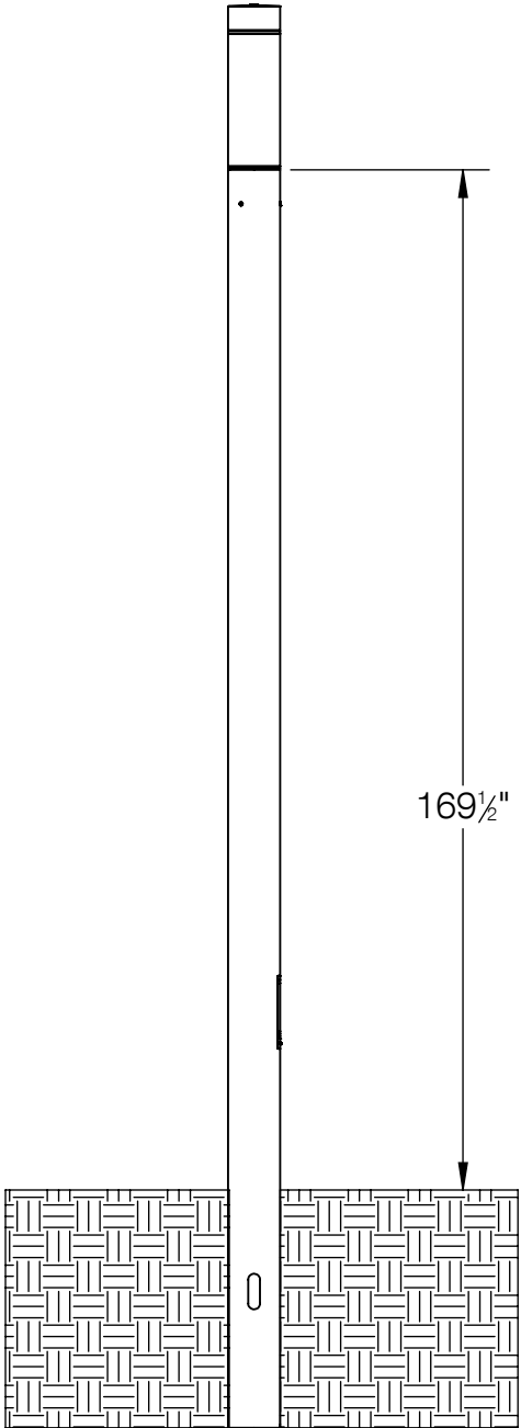
84720 SYSTEM BUILDING ELEMENT POLE SHOWN WITH SYSTEM BUILDING ELEMENT HEAD 84817 (NOT TO SCALE, HEAD SOLD SEPERATELY)
