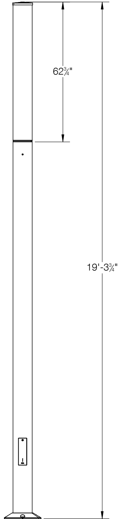
84734 SYSTEM BUILDING ELEMENT HEAD SHOWN ON SYSTEM BUILDING ELEMENT POLE 84721 (NOT TO SCALE, POLE SOLD SEPERATELY)
