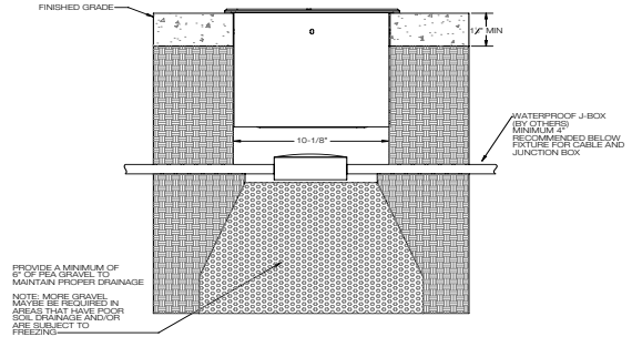
Figure 1: Mounting
