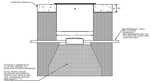
Figures 2 & 3: Installation Clamping System
