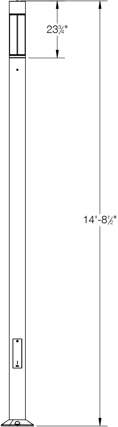
84816 SYSTEM BUILDING ELEMENT HEAD SHOWN ON SYSTEM BUILDING ELEMENT POLE 84713 (NOT TO SCALE, POLE SOLD SEPERATELY)
