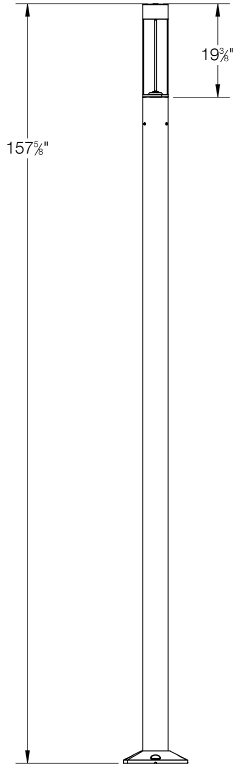
84818 SYSTEM BUILDING ELEMENT HEAD SHOWN ON SYSTEM BUILDING ELEMENT POLE 84709 (NOT TO SCALE, POLE SOLD SEPERATELY)
