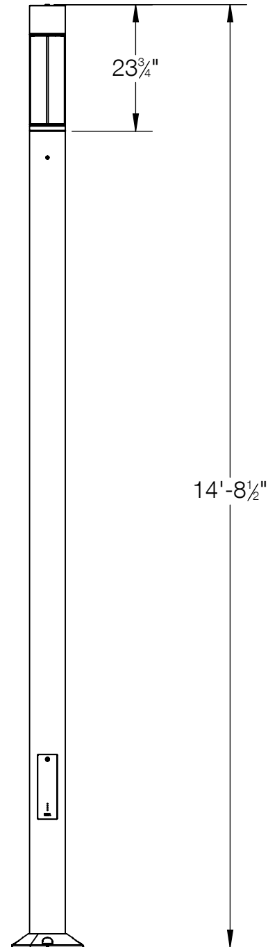
84819 SYSTEM BUILDING ELEMENT HEAD SHOWN ON SYSTEM BUILDING ELEMENT POLE 84713 (NOT TO SCALE, POLE SOLD SEPERATELY)
