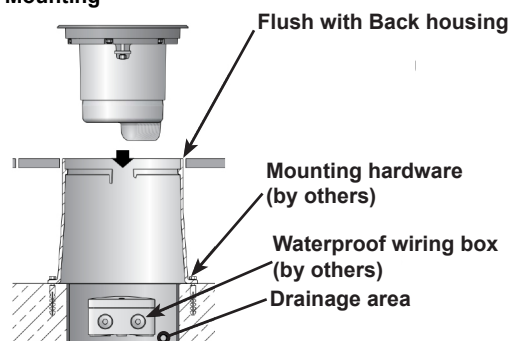
Figure 2: Faceplate Detail
