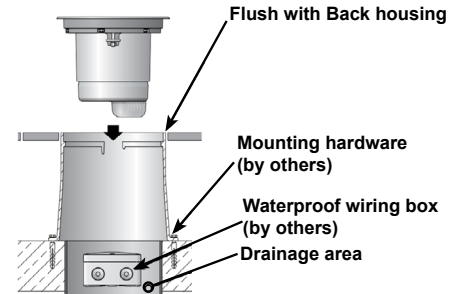
Figure 2: Faceplate Detail
