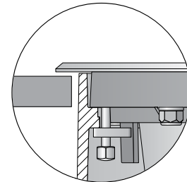
Figure 3: Optical Assembly Adjustment (Generic Image)
