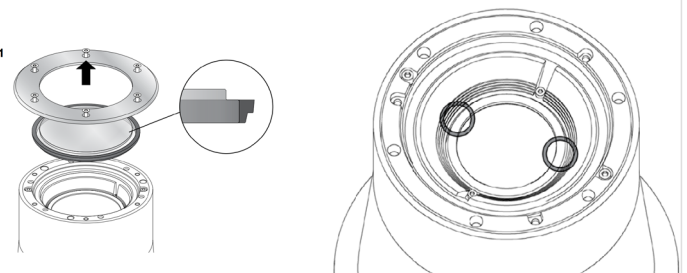
Figure 3: Optical Assembly Adjustment (Generic Image)
