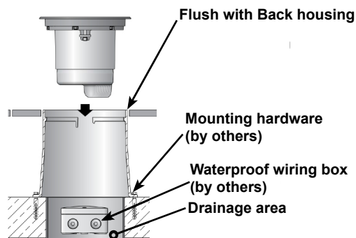
Figure 1: Mounting
