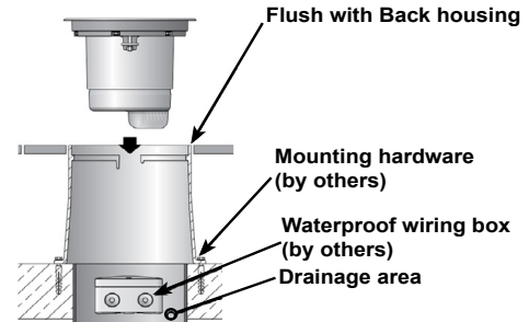
Figure 2: Faceplate Detail
