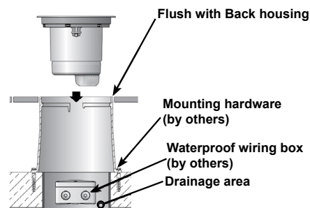
Figure 2: Faceplate Detail
