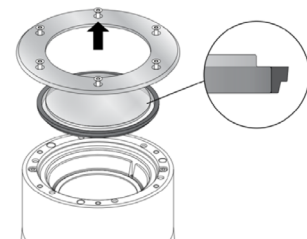
Figure 4: Faceplate Removal (Generic Image)
