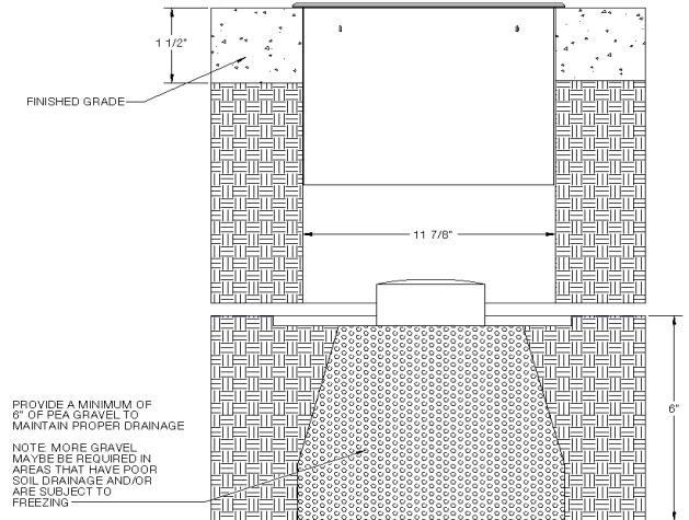
Figures 2 & 3: Installation Clamping System
