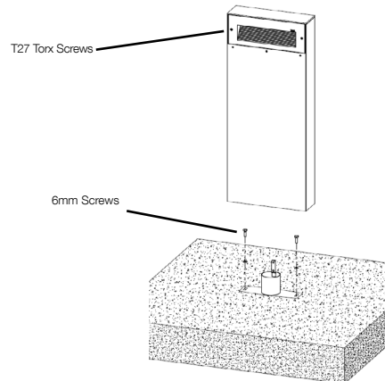
Figure 2: Bottom View
