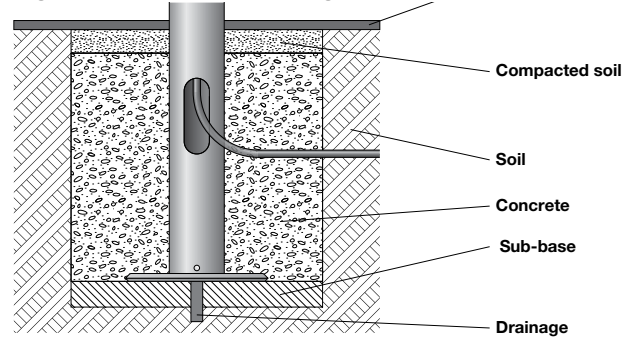
Figure 2: Example mounting
