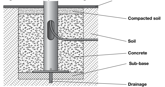
Figure 2: Example mounting
