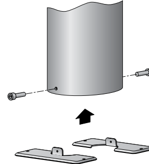
Figure 2: Example mounting
