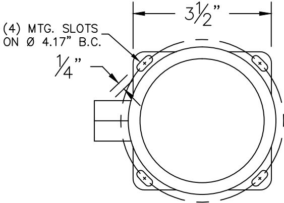
MOUNTING DETAIL (TOP VIEW WITHOUT TOP)
