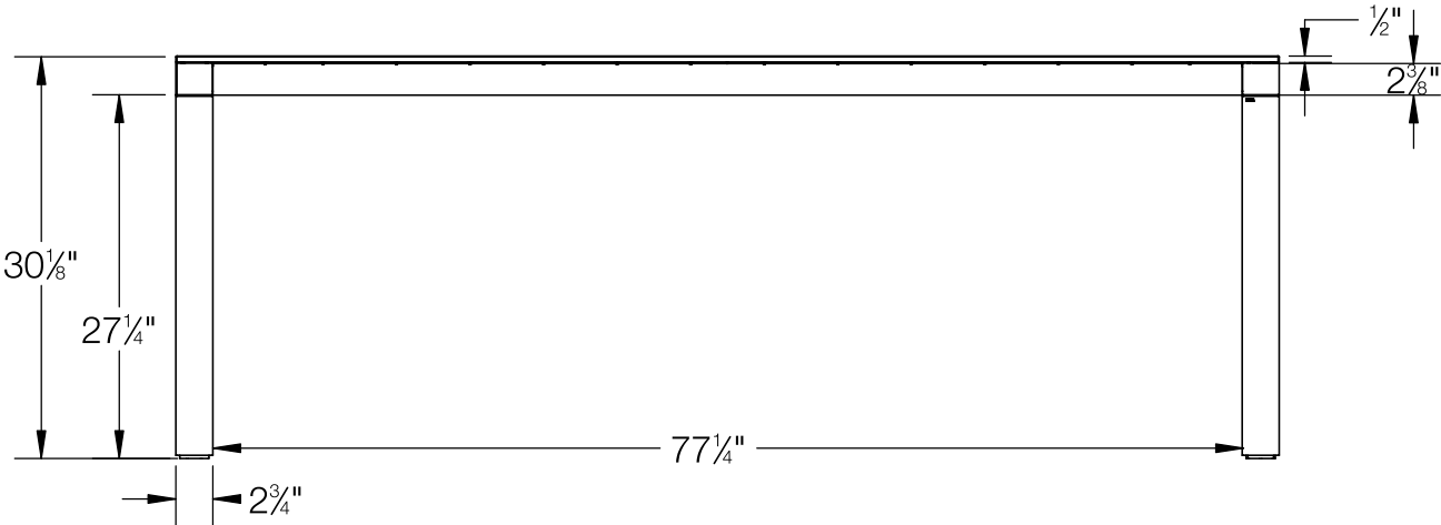
FRONT VIEW
