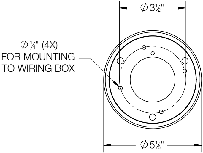
MOUNTING PLATE DETAIL
