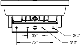
Figure 1: Yolk Mounting Detail
