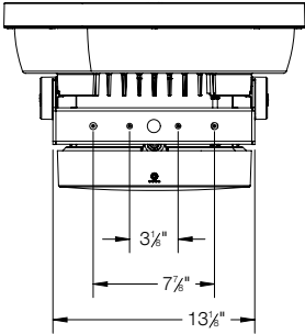
Figure 1: Yolk Mounting Detail
