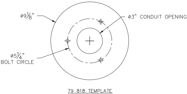
Figure 1: Anchorage Template
