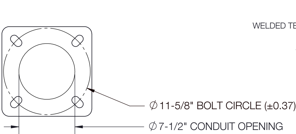
BASE DETAIL NOT TO SCALE
