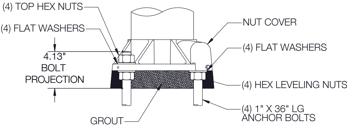
ANCHOR DETAIL
